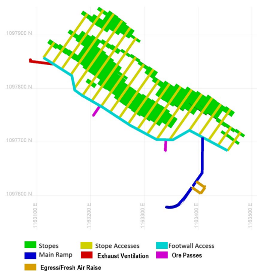
Figure 16.12 Lower Mine typical level plan
