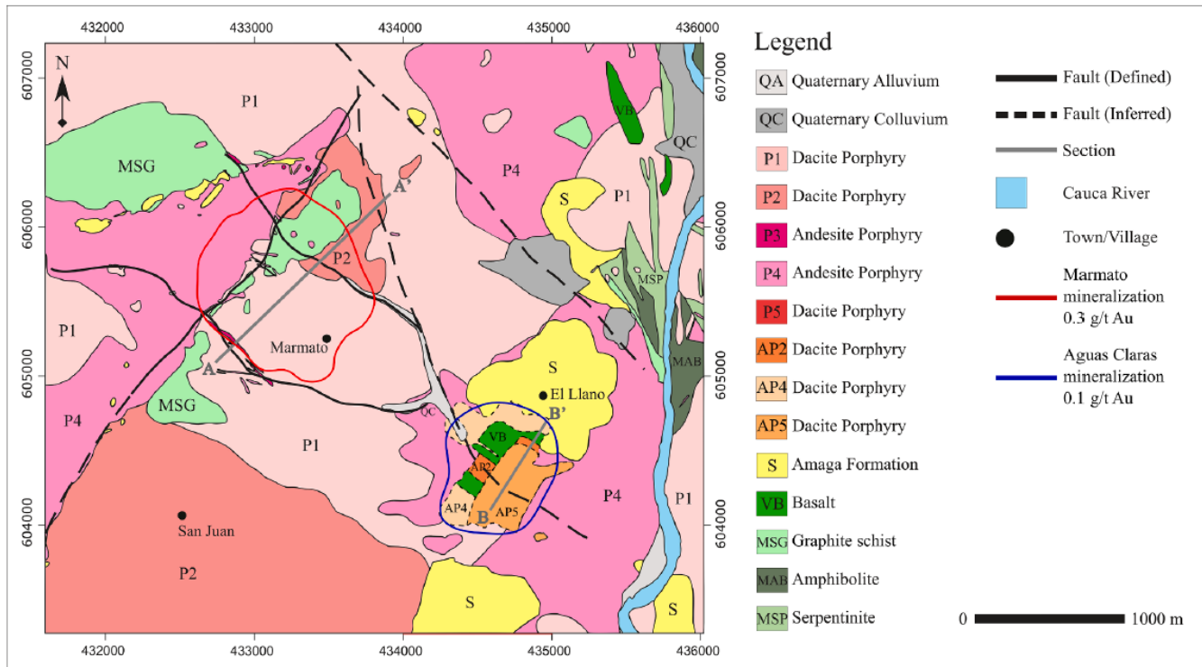
Figure 7.2 Local geology plan
