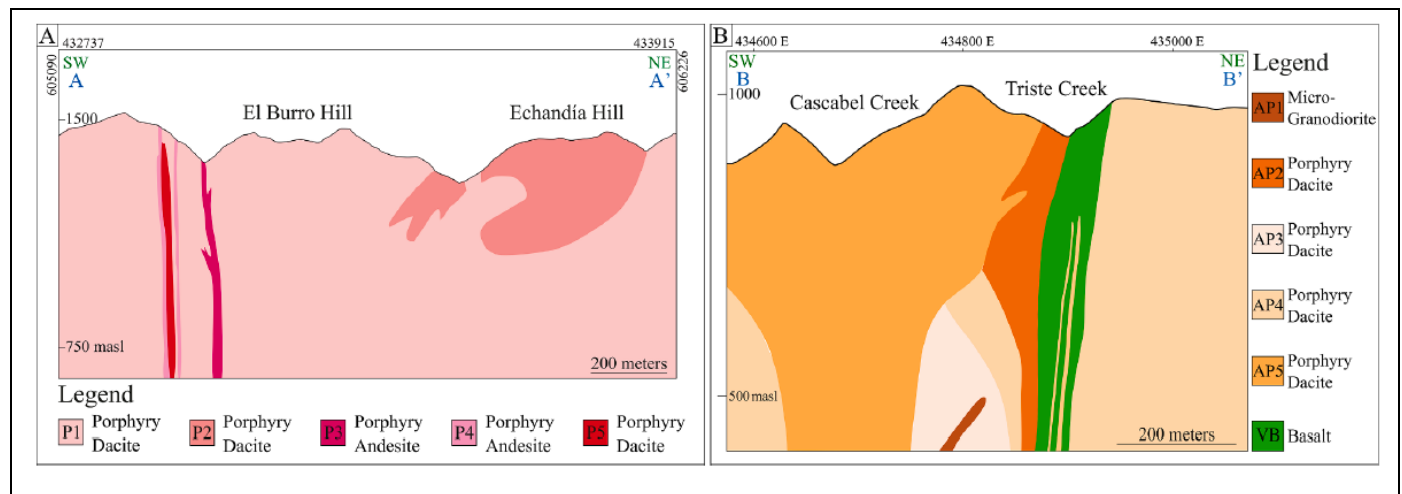
Figure 7.3 Property geology cross sections
